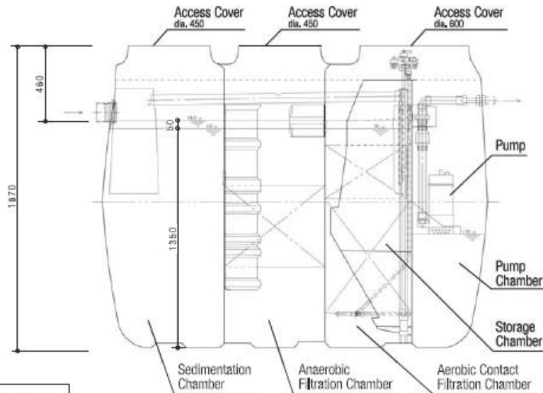
Vertical Sectional View
